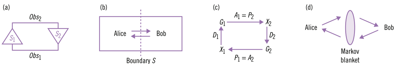
Figure 1 • Four representations of two-agent, or alternatively, agent-environment interaction. (a) Two agents S_1 and S_2 , here depicted as computational processes, exchange observations Obs_1 and Obs_2 (adapted from Foerster 1976: 94). (b) Two agents, or alternatively two classical black boxes, Alice and Bob exchange inputs and outputs across a boundary S that is in principle arbitrarily movable as described in Fields (2016). Alice's outputs are Bob's inputs and vice versa. (c) Two conscious agents as defined by Hoffman and Prakash (2014) act on each other. Here X_1 and G_1 and X_2 and G_2 are measurable spaces representing the experiences and available actions, respectively, of the two agents; D_1 and D_2 , P_1 and P_2 , and A_1 and A_2 are Markov kernels representing the decision processes, perceptions, and executed actions, respectively, of the two agents. (d) Two agents interact via an intervening Markov blanket as described in Friston (2013). Arrows represent Markov processes.
