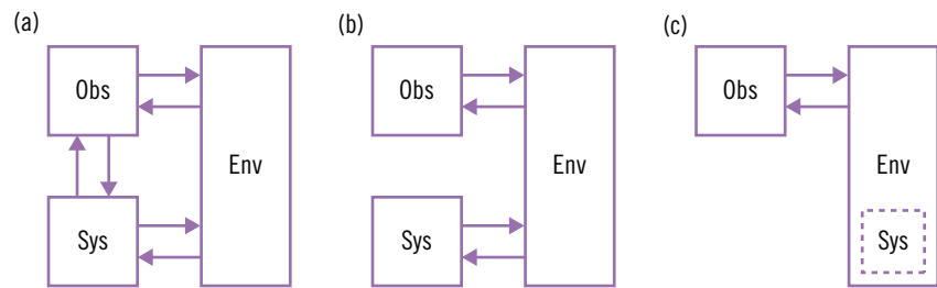
Figure 2 • Three views of decoherence. (a) An observer (Obs) prepares and measures a quantum system (Sys). Both independently interact with a large surrounding environment (Env), which renders their states effectively classical by a decoherence mechanism (e.g., ambient photon scattering). (b) The “environment as witness” formulation of Ollivier, Poulin & Zurek (2004, 2005), in which the observer interacts with the system only via the “witnessing” environment. This environment decoheres the system but interacts effectively classically with the observer. (c) If the assumption of environmental transparency is rejected, the environment becomes a black box. In this case, the system is completely embedded within it in a way that provides the observer with no access to the system-environment boundary. In this case, decoherence can only be defined at the observer-environment boundary.
