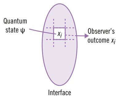
Figure 3 • Decoherence encodes a classical outcome value x_i on the observer-environment interface. Such an encoding is required if receipt of the observational outcome is to be considered to have any effect on the observer's subsequent behavior. This encoding is holographic, i.e., the only information about the environment that the observer can obtain is the information that can be encoded on the observer-environment interface by decoherence.
