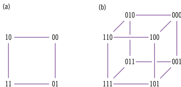
Figure 6 • Binary codes with redundancies of (a) two and (b) three. Each line represents one bit flip and hence a Hamming distance of one. The codes “00” and “11” are a Hamming distance of two apart, while “000” and “111” are a Hamming distance of three apart. Receiving “10” or “01” provides no information about the intended message, while receiving “110,” “101” or “011” suggests “111” and receiving “100,” “010” or “001” suggests “000.” Hence the three-bit code provides error correction while the two-bit code does not.
