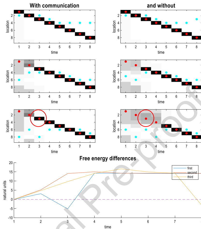
Figure 5 – Simulations of active inference. The upper panels depict posterior beliefs—about the location of the subject—as posterior distributions over the nine possible locations (columns) at each of the (eight) timesteps. The right-hand panels reproduce the belief updating shown in the left hand panels but in the absence of communication. Each panel reports the posterior beliefs as a function of time along the x-axis. The beliefs in this case are probability distributions over nine locations, shown as a greyscale image. In other words, uncertain, imprecise beliefs correspond to grey regions that cover multiple locations. Over time, uncertainty is resolved, and beliefs becomes very precise with a concentration of probability in the black regions. The true location is shown by the red dots, while the cyan dots indicate where the agent was looking. Note that these locations are restricted to the agent’s line of sight—and one location to the right and left. The three rows of panels report the belief updating for the three agents. The left panels show belief updating with communication. The three panels on the right show the corresponding active inference in the absence of communication, using the same sequence of hidden states. Communication or language was suppressed by rendering the auditory likelihood mappings very imprecise. The lower panel shows differences in free energy as a function of time for the three agents (coloured lines), when comparing belief updating with and without communication. The red circle highlights the epoch of belief updating illustrated in the next figure. This epoch illustrates the benefits of communication in the sense that the third agent has resolved her uncertainty about the location of the subject by the third epoch, whereas the same agent without communication only forms precise beliefs, after seeing the subject at the fifth epoch.
